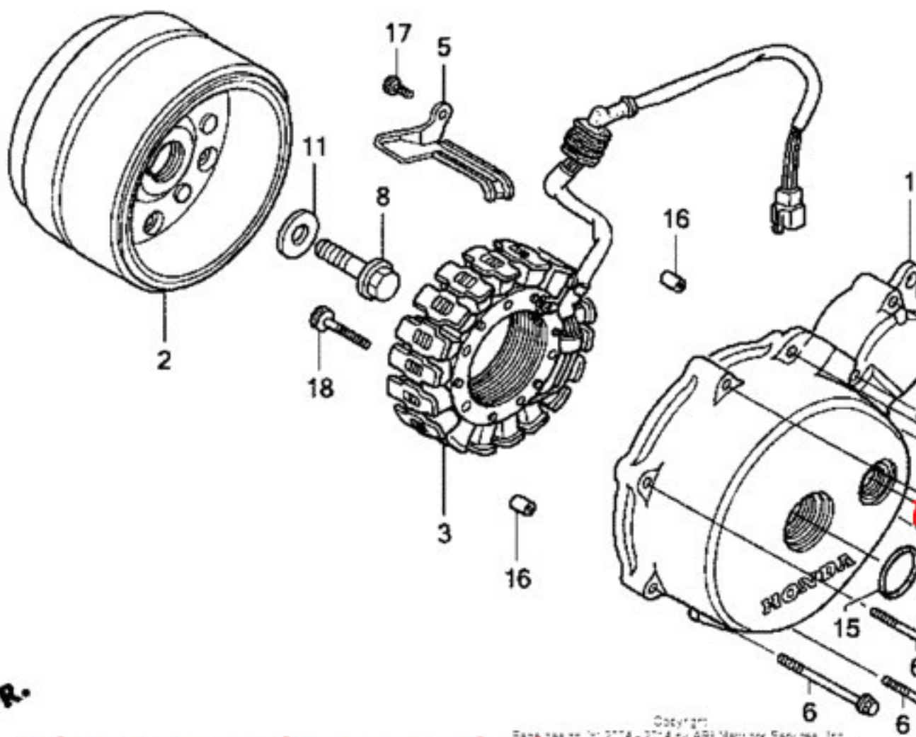
Schemat: Honda VF750 Shadow RC44
